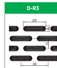
Hole Size: Oblong 6.0x25.0mm Pitch: 11.0x30.0mm Open Area: 45.0%
