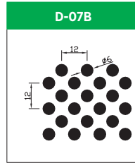
Hole Size: Dia. 6.0mm Pitch: 12.0mm Open Area: 39.0%
