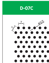
Hole Size: Dia. 3.5mm Pitch: 7.0mm Open Area: 23.0%
