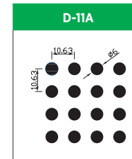
Hole Size: Dia. 6.0mm Pitch: 10.63mm Open Area: 25.0%
