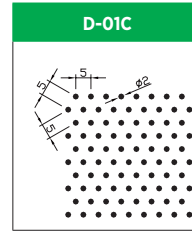
Hole Size: Dia. 2.0mm Pitch: 5.0mm Open Area: 29.0%
