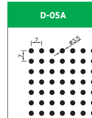
Hole Size: Dia. 3.5mm Pitch: 7.0mm Open Area: 20.0%
