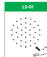
Hole Size: Dia. 2.5mm Pitch: 10.0mm Open Area: 5.0%
