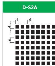
Hole Size: Q.S. 4.0x4.0mm Pitch: 6.0x6.0mm Open Area: 44.0%
