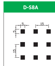
Hole Size: Q.S. 5.0x5.0mm Pitch: 15.0x15.0mm Open Area: 11.0%
