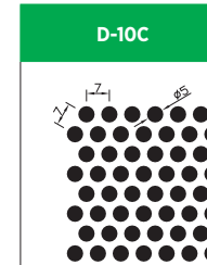
Hole Size: Dia. 5.0mm Pitch: 7.0mm Open Area: 46.0%
