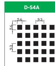
Hole Size: Q.S. 5.6x5.6mm Pitch: 9.3x9.3mm Open Area: 36.0%
