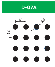
Hole Size: Dia. 6.0mm Pitch: 12.0mm Open Area: 20.0%
