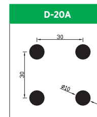
Hole Size: Dia. 100mm Pitch: 30.0mm Open Area: 9.0%
