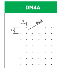
Hole Size: Dia. 0.8mm Pitch: 7.0mm Open Area: 1.0%
