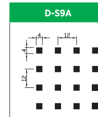
Hole Size: Q.S. 4.0x4.0mm Pitch: 12.0mm Open Area: 11.0%
