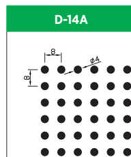
Hole Size: Dia. 4.0mm Pitch: 8.0mm Open Area: 20.0%
