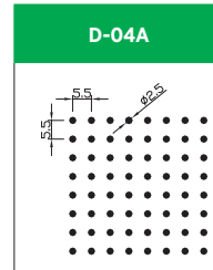
Hole Size: Dia. 2.5mm Pitch: 5.5mm Open Area: 16.0%
