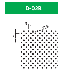
Hole Size: Dia. 1.8mm Pitch: 5.0mm Open Area: 20.0%
