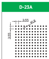
Hole Size: Dia. 1.8mm Pitch: 3.55mm Open Area: 20.0%
