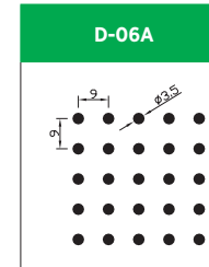
Hole Size: Dia. 3.5mm Pitch: 9.0mm Open Area: 12.0%
