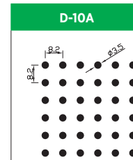
Hole Size: Dia. 3.5mm Pitch: 8.2mm Open Area: 14.0%
