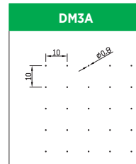
Hole Size: Dia. 0.8mm Pitch: 1.0mm Open Area: 0.5%
