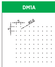
Hole Size: Dia. 0.8mm Pitch: 5.0mm Open Area: 2.0%
