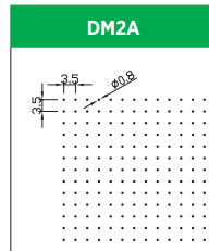
Hole Size: Dia. 0.8mm Pitch: 3.5mm Open Area: 4.0%
