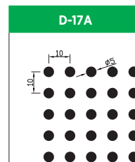
Hole Size: Dia. 5.0mm Pitch: 10.0mm Open Area: 20.0%
