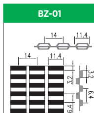
Hole Size: Oblong 3.2x11.4mm Pitch: 6.4x14mm Open Area: 40.71%
