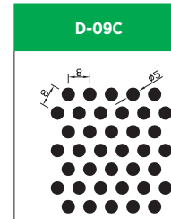
Hole Size: Dia. 5.0mm Pitch: 8.0mm Open Area: 35.0%
