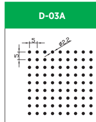
Hole Size: Dia. 2.2mm Pitch: 5.0mm Open Area: 15.0%
