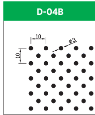
Hole Size: Dia. 3.0mm Pitch: 10.0mm Open Area: 14.0%
