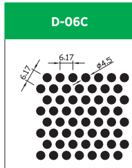
Hole Size: Dia. 4.5mm Pitch: 6.17mm Open Area: 48.0%
