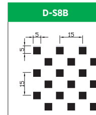
Hole Size: Q.S. 5.0x5.0mm Pitch: 15.0mm Open Area: 22.0%
