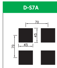
Hole Size: Q.S. 45.0x45.0mm Pitch: 7.0x7.0mm Open Area: 41.0%
