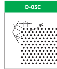
Hole Size: Dia. 2.0mm Pitch: 4.0mm Open Area: 23.0%
