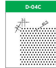
Hole Size: Dia. 1.5mm Pitch: 3.1mm Open Area: 21.0%
