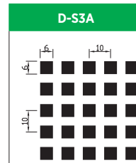
Hole Size: Q.S. 4.0x4.0mm Pitch: 10.0x10.0mm Open Area: 36.0%
