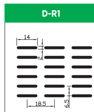
Hole Size: Oblong 2.0x14.0mm Pitch: 6.5x18.5mm Open Area: 23.0%
