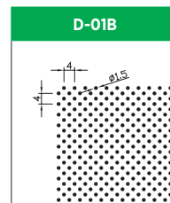
Hole Size: Dia. 1.5mm Pitch: 4.0mm Open Area: 22.0%
