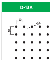
Hole Size: Dia. 3.0mm Pitch: 10.0mm Open Area: 7.0%
