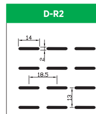
Hole Size: Oblong 2.0x14.0mm Pitch: 13.0x18.5mm Open Area: 11.0%
