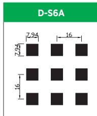
Hole Size: Q.S. 7.94x7.94mm Pitch: 16mm Open Area: 25.0%
