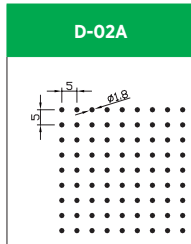
Hole Size: Dia. 1.8mm Pitch: 5.0mm Open Area: 10.0%
