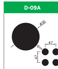
Hole Size: Dia. 30.0mm Pitch: 47.0mm Open Area: 32.0%
