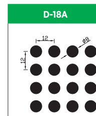
Hole Size: Dia. 8.0mm Pitch: 12.0mm Open Area: 35.0%
