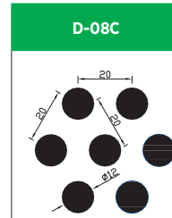
Hole Size: Dia. 12.0mm Pitch: 20.0mm Open Area: 33.0%
