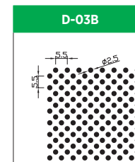
Hole Size: Dia. 2.5mm Pitch: 5.5mm Open Area: 32.0%
