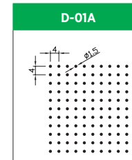
Hole Size: Dia. 1.5mm Pitch: 4.0mm Open Area: 11.0%
