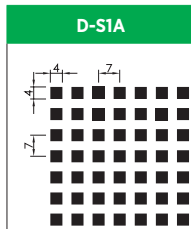
Hole Size: Q.S. 4.0x4.0mm Pitch: 7.0x7.0mm Open Area: 33.0%
