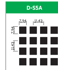
Hole Size: Q.S. 7.94x7.94mm Pitch: 11.43x11.43mm Open Area: 48.0%
