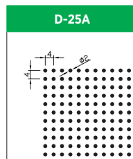
Hole Size: Dia. 2.0mm Pitch: 4.0mm Open Area: 20.0%
