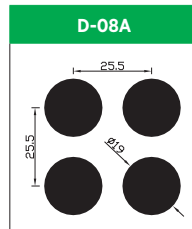
Hole Size: Dia. 19.0mm Pitch: 25.5mm Open Area: 44.0%
