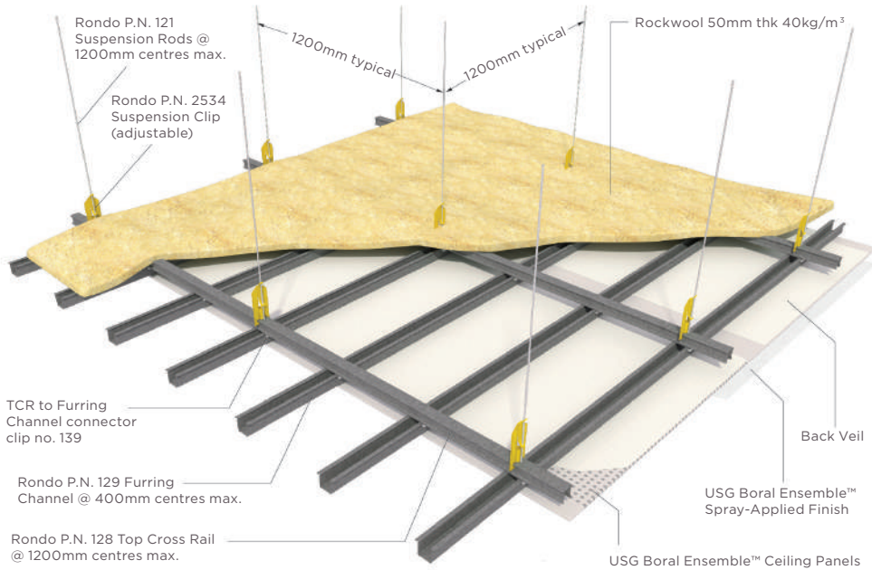
USG Boral Ensemble™ Seamless Acoustical Plasterboard Ceiling System
